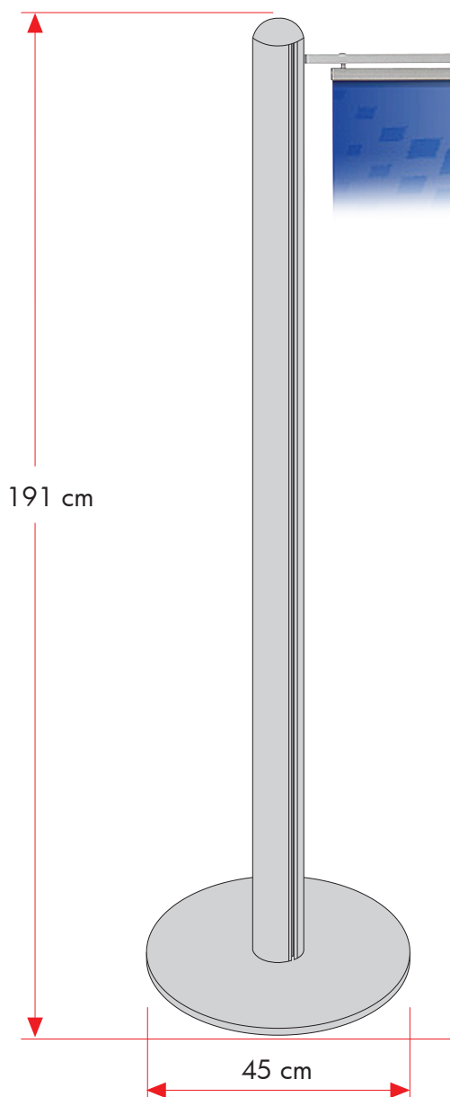
Poster Hanger Profiles for banner width 40/50/60/70 cm. Max. banner height 180 cm.
